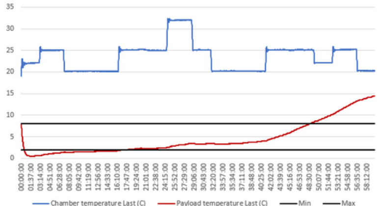
PROVEN PERFORMANCE - AFNOR Summer Profile | 3L
