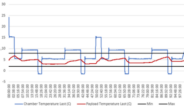
PROVEN PERFORMANCE - AFNOR Winter Profile | 3L
